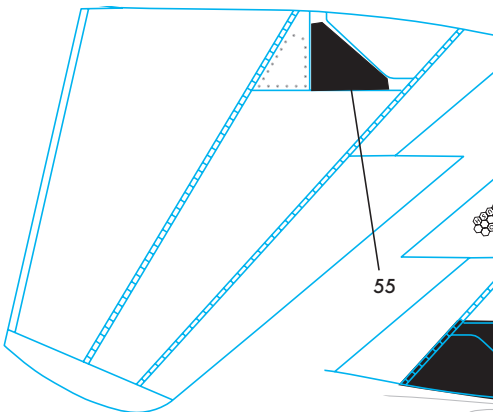
Bottom side left stabilizer
