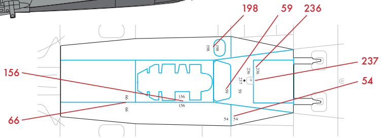
Bottom side left stabilizer
